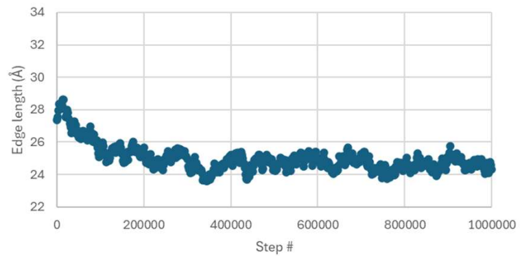
0.5 ns NPT Cell Dimension w/ 2 constrained atoms
