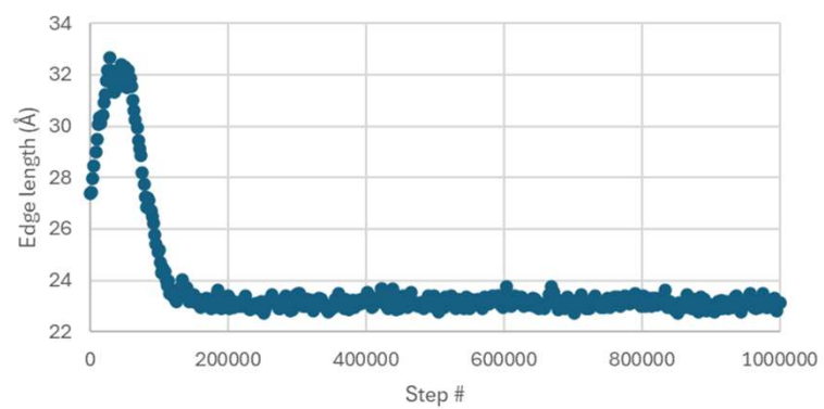
0.5 ns NPT Cell Dimension 0 constrained atoms
