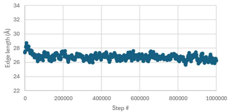
0.5 ns NPT Cell Dimension w/ 3 constrained atoms
