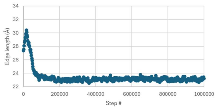
0.5 ns NPT Cell Dimension 1 constrained atoms
